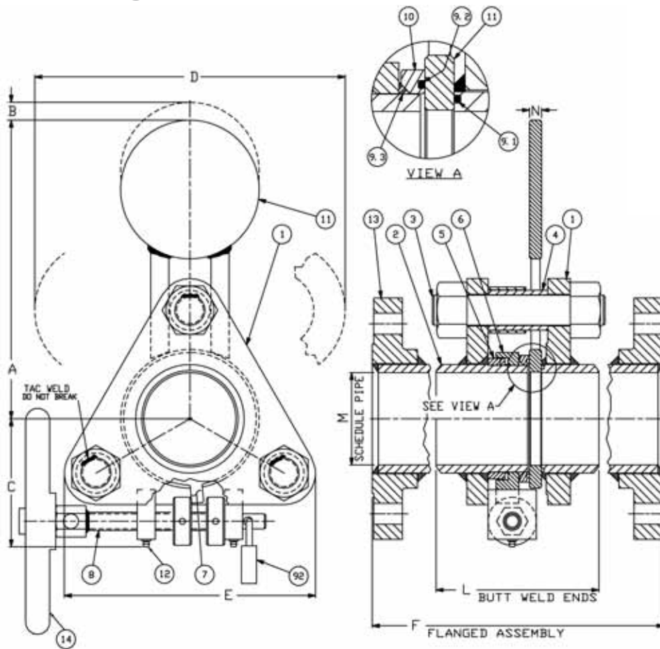
Cam-Set® front view
